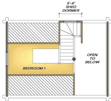
Upper Level floor Plan
